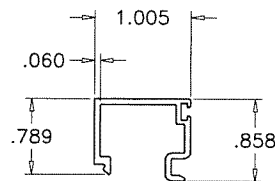
5 GLAZING STOP
