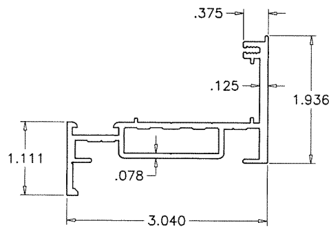
1 FLANGE FRAME HEAD/SILL/JAMB
