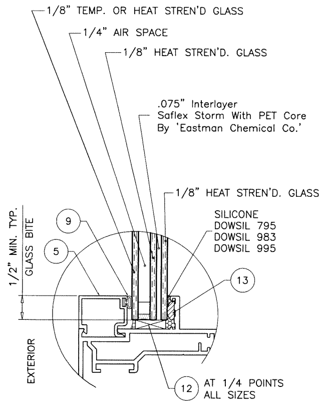
GLASS TYPE 'Ai' 11/16" OVERALL INSUL. LAM. GLASS
