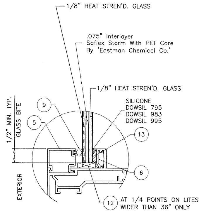
GLASS TYPE 'A' 5/16" OVERALL LAM. GLASS
