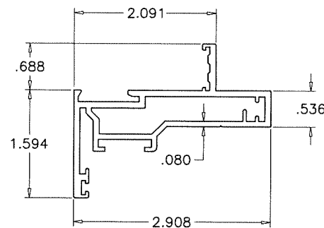
2 VENT TOP/BOTTOM/SIDE RAIL
